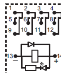
DC, with fly-wheel diode
